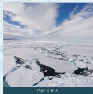
PACK ICE
